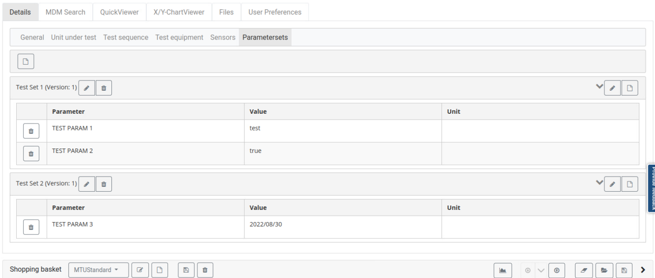
Figure 16. Parametersets overview
