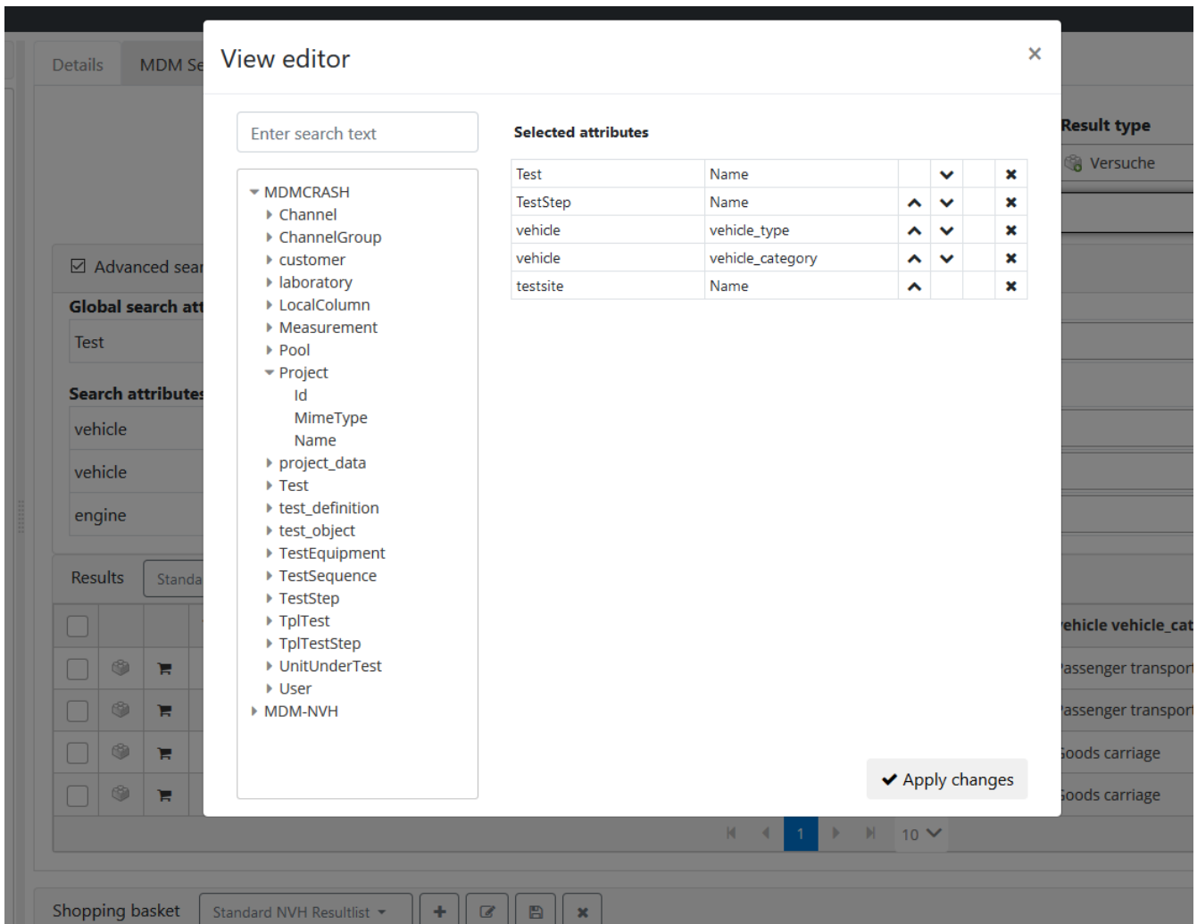
Figure 12. View Editor
