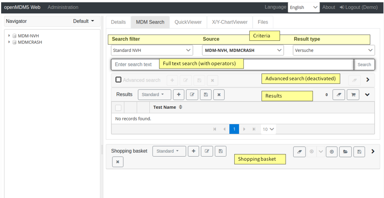
Figure 5. MDM Search
