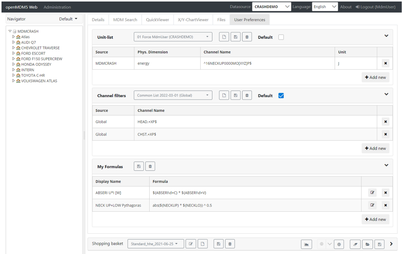
Figure 22. User Preferences
