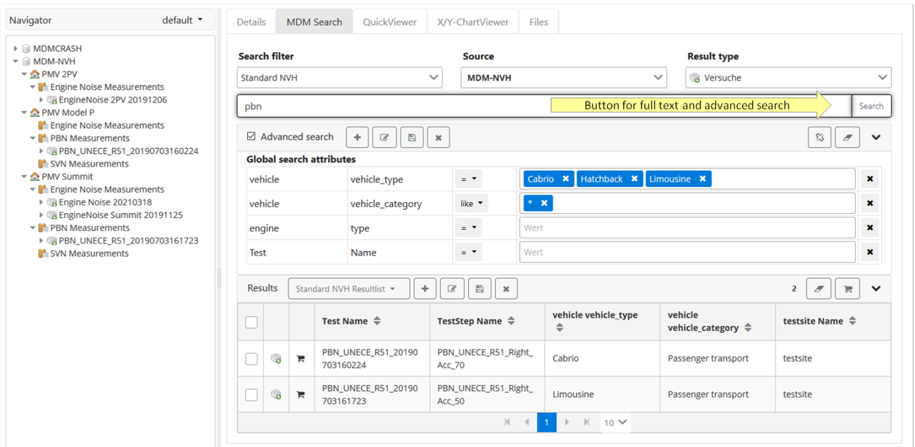
Figure 9. MDM Search
